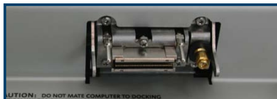
CAUTION: DO NOT MATE COMPUTER TO DOCKING HEAD CONNECTOR. Docking Head Connector shown in the activated 'DOCK' position without a docked computer in place.
